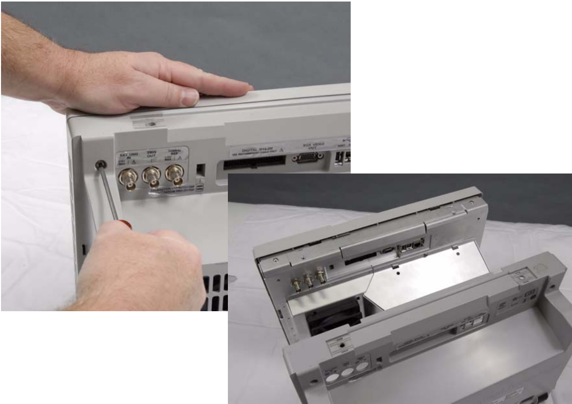
Figure 18 Removing cabinet
